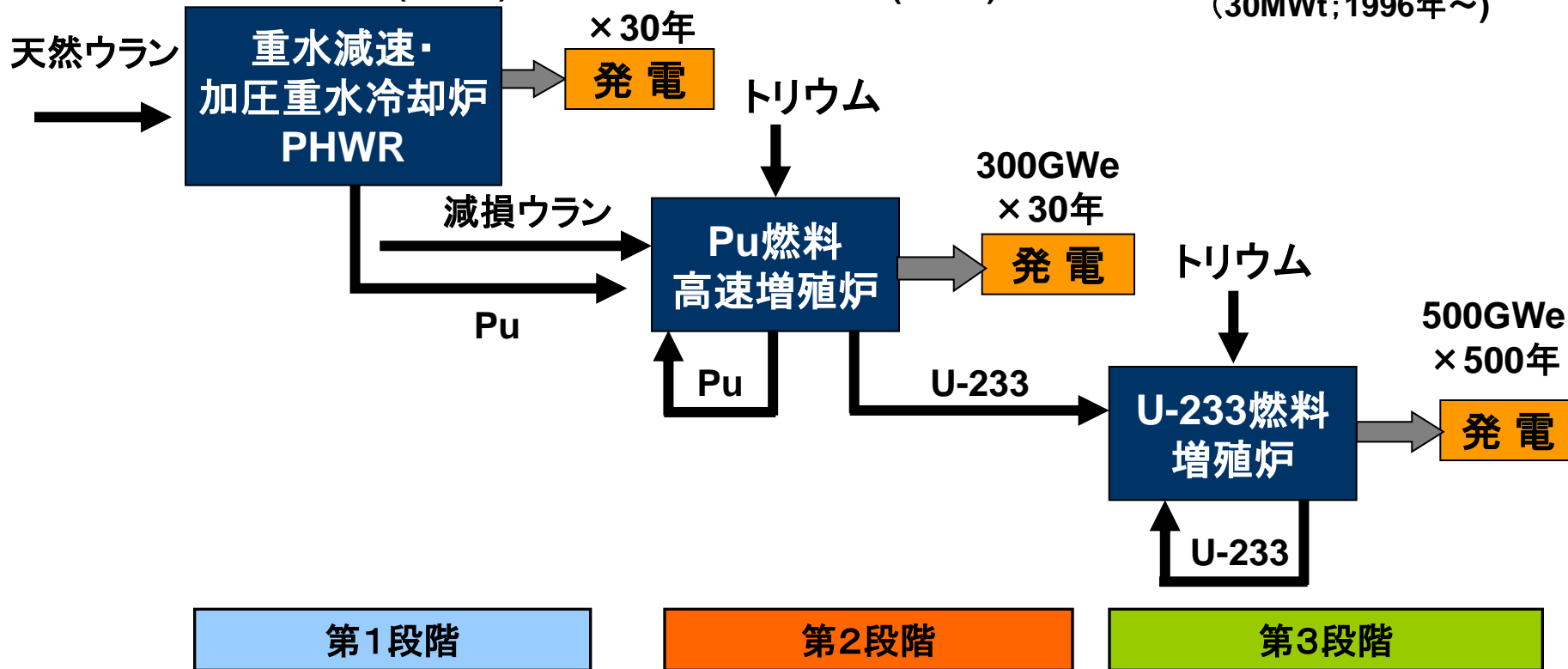
U-235 (MAPS)
